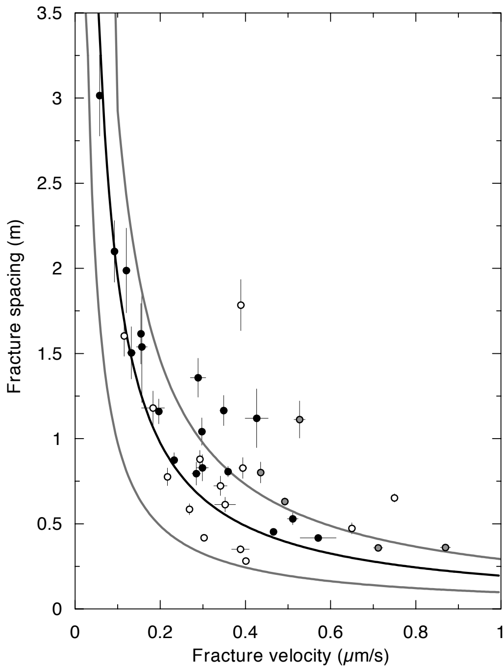
Figure 4.4: The average fracture front velocity and fracture spacing are inversely related in joints in lava. The fracture spacings from field observations in the tholeiitic basalts of the Columbia River Basalt Group (black circles), and the island of Staffa (grey circles), and from a range of columnar lavas types found in southwestern British Columbia (open circles) are shown. Solid lines indicate an inverse dependence of fracture spacing on fracture velocity, with lines of constant Péclet number Pe = 0.15 , 0.3 , and 0.5 shown.
