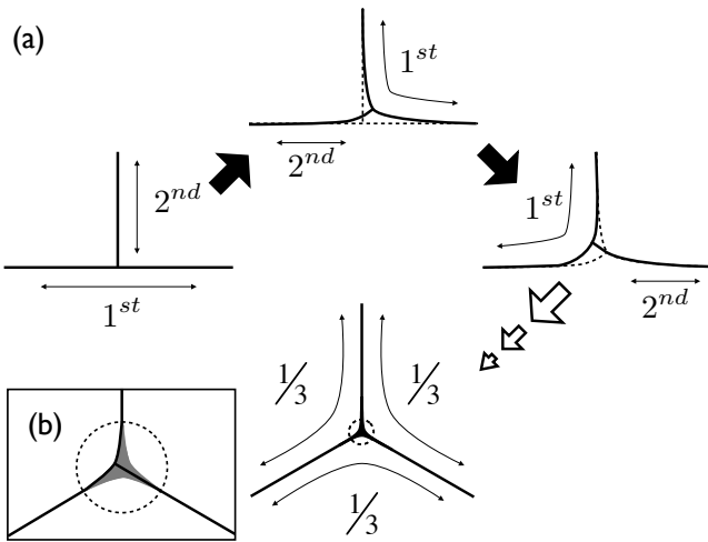
FIG. 9: The crack pattern in a clay layer changes when the layer is repeatedly wetted and dried. (a) A T-junction (left) contains information about the order of crack formation, as a later crack will intersect an earlier crack at right angles. In different generations (progressing clockwise), the order of cracks can differ, encouraging adjustments in the crack pattern. After many generations (bottom), if each crack path is equally likely to form first, symmetry suggests a Y-junction. (b) Very close to the vertex of a Y-junction, the cracks may still curve, in response to the order of crack formation in any particular generation. Over all possible paths, these changes will cancel out for a Y-junction. However, for a T-junction, the vertex will move, on average, as indicated in (a). Compare the process sketched here to that observed in Fig. 2.
