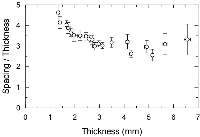
FIG. 3: The spacing of desiccation cracks in bentonite clay increases as the thickness of the cracking layer increases. For thin layers with unconnected cracks the crack spacing appears to be larger than expected from a simple proportional relationship.
