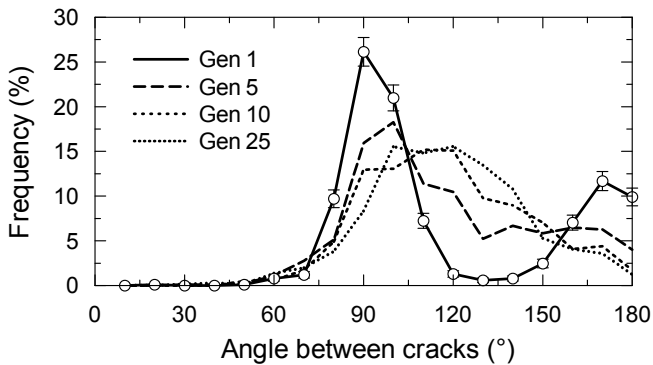
FIG. 6: The distribution of joint angles in clay layers changes with repeated cycles of wetting and drying. The distribution is peaked at 90^\circ and 180^\circ in the initial pattern, but tends towards 120^\circ after repeated dryings. Representative error bars are shown on Generation 1, and all data are averaged over 10^\circ bins.
