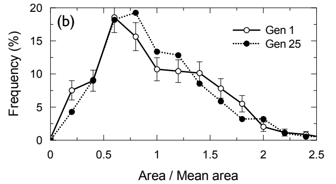
FIG. 5: The average cross-sectional area of clay cells increases slightly in the first 5 generations, as some cracks will not be open in any particular generation. However, histograms of the distributions of cell areas do not show any other substantial differences between the 1st and 25th generations. Representative error bars are shown for Generation 1.
