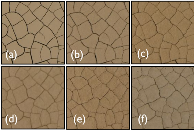
FIG. 4: The pattern of cracks changes slowly after many cycles of wetting and drying. The initial pattern (a) is dominated by cracks meeting at 90^\circ and 180^\circ . Through generations (b) 3, (c) 5, (d) 10, (e) 15, and (f) 25, the pattern slowly changes to one with many joints closer to 120^\circ angles. Each panel shows a 6 \times 6 \text{ cm}^2 area at the centre of a dried bentonite slurry.
