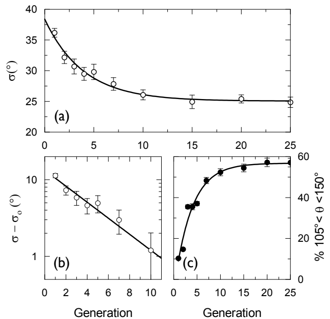
FIG. 7: (a) The standard deviation of joint angles, \sigma , decreases rapidly within the first 10 generations, to a final value \sigma_o . (b) An exponential decrease towards \sigma_o is well-fitted to the data, with a decay time of 4.2 \pm 0.5 generations. (c) The proportion of angles close to 120^\circ also shows an exponential relaxation, with a decay time of 3.7 \pm 0.6 generations.
