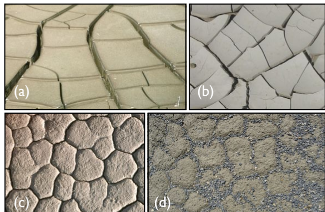
FIG. 1: There are a variety of fracture patterns commonly found in dried mud. (a,b) show rectilinear patterns, where cracks typically meet at ‘T-junctions’ of 90^\circ and 180^\circ . (c,d) show, in contrast, hexagonal patterns, where cracks meet at ‘Y-junctions’ of 120^\circ . [Panels (a,c) courtesy of B. Hallet.]
